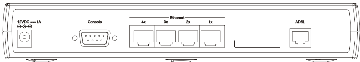
Rear Panel
