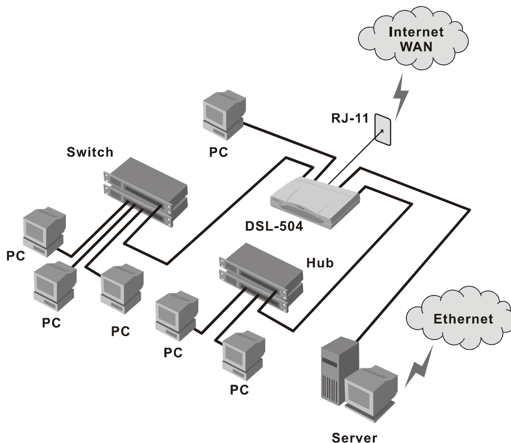
LAN to Router Connection
