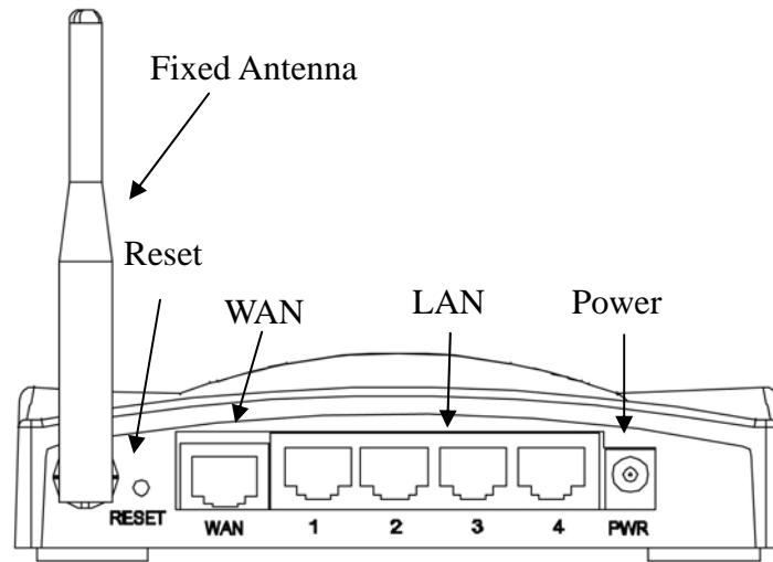
Figure 2 – WLAN Broadband Router Rear Panel (Fixed Antenna)
