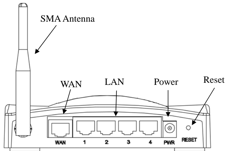
Figure 2.1 – WLAN Broadband Router Rear Panel (SMA Antenna)
