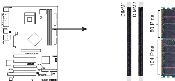
P4P800S SE 184-Pin DDR DIMM Sockets
