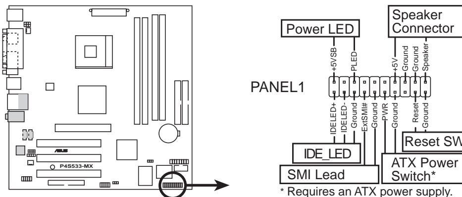
P4S533-MX System Panel Connectors
