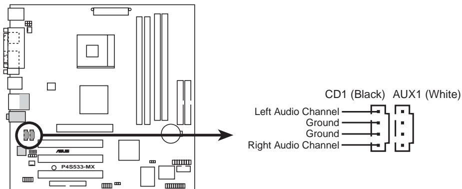
P4S533-MX Internal Audio Connectors
