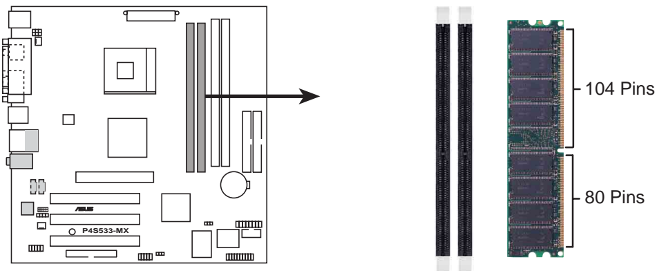
P4S533-MX 184-Pin DDR DIMM Sockets
