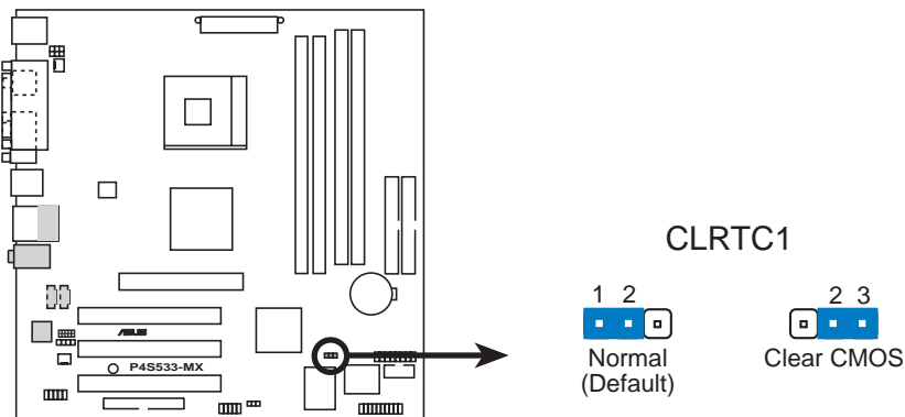
P4S533-MX Clear RTC RAM Setting
